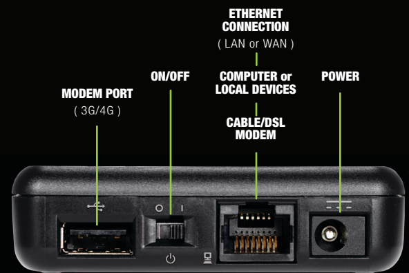
CradlePoint CTR35
